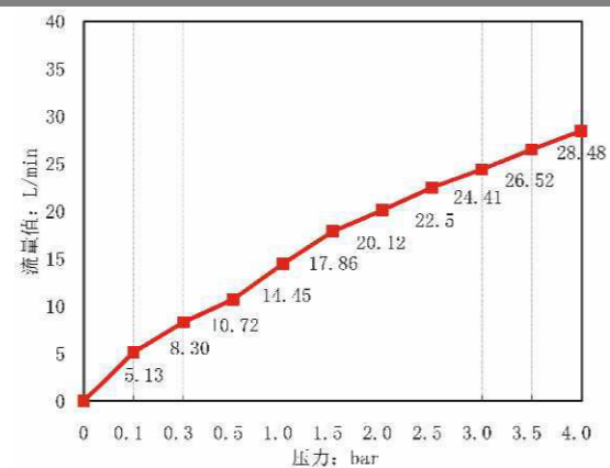
流量图 Flow Rate Curves
